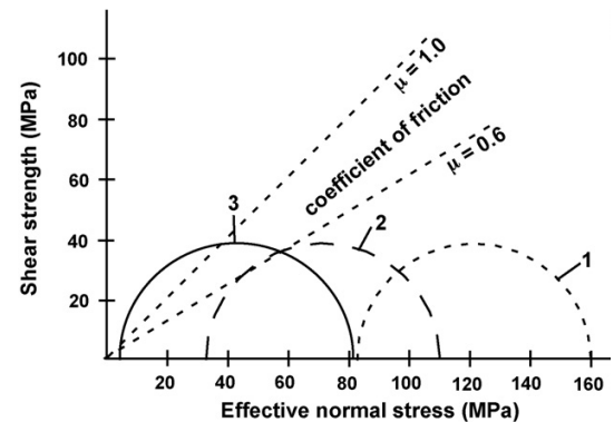
Figure 7. Mohr diagram illustrating the effect of increasing pore pressure in weak rock. Circle 1 is total stress, Circle 2 is effective stress at hydrostatic conditions, and Circle 3 is effective stress at maximum overpressure conditions during hydraulic stimulation (Haring et al., 2008).
