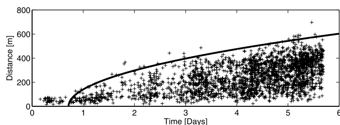
Figure 8. Injection pressure, flow rate and an r - t plot of the corresponding fluid injection microseismicity at a geothermal borehole in Basel region of Switzerland. The data are courtesy of U. Schanz and M.O Haring. Curve is Equation (7) with D = 0.06 \text{ m}^2/\text{s} . From Shapiro et al., (2009).
