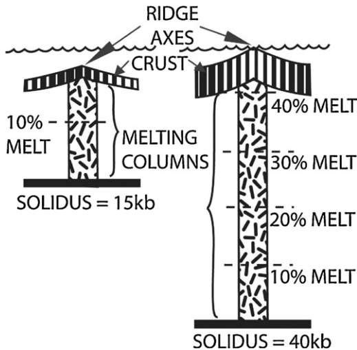
Fig. 11. The Global Systematics model. Left: low T_p , deep bathymetry, thin crust, high \text{Na}_8 and low \text{Fe}_8 . Right: high T_p , shallow bathymetry, thick crust, low \text{Na}_8 and high \text{Fe}_8 .
