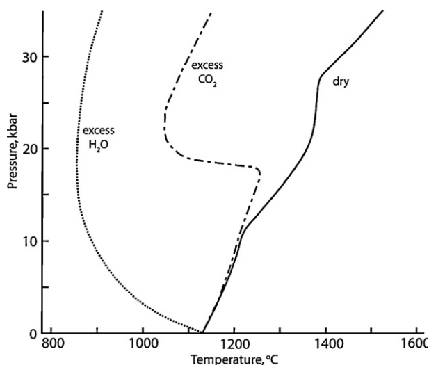
Fig. 5. The effect of volatiles on the solidus temperature of peridotite.
