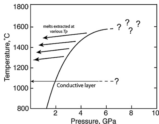
Fig. 1. Schematic diagram showing the thermal conditions in the shallow Earth. Melts drawn from deeper within the conductive layer have higher T_p than those drawn from shallower.
