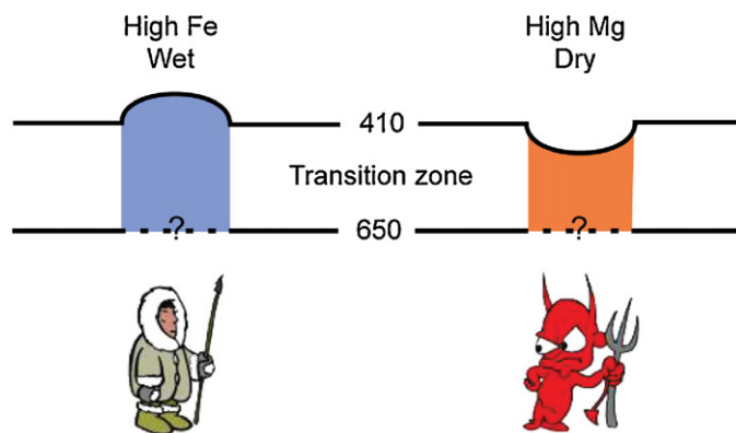
Fig. 9. The effect on the transition zone discontinuities of composition, water content, and temperature.
