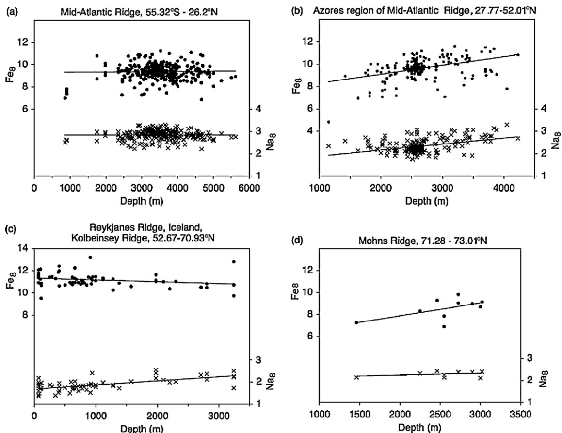
Fig. 19. \text{Na}_8 and \text{Fe}_8 vs. depth for different sections of the Mid-Atlantic Ridge.
