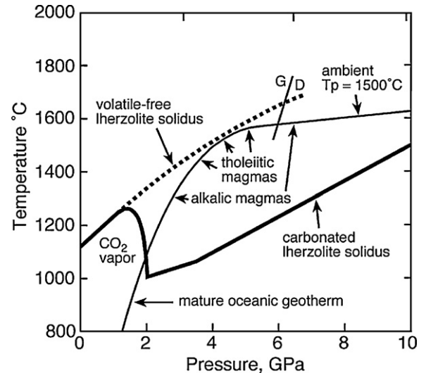
Fig. 6. Solidus curves for carbonated lherzolite and volatile-free lherzolite. G, graphite; D, diamond.
