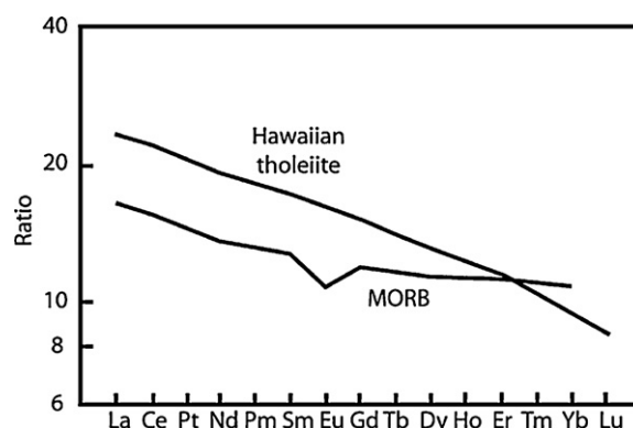
Fig. 14. Rare-earth-element concentration ratios with respect to depleted mantle for normal MORB and Hawaiian tholeiite.
