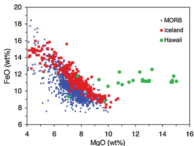
Fig. 24. Plot of wt% FeO vs. wt% MgO for basalt glass from mid-ocean ridges, Iceland and Hawaii (G. Gudfinnsson, unpublished).
