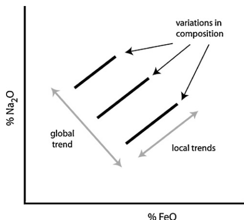
Fig. 18. Variations in %Na 2 O vs. %FeO predicted by laboratory experiments to occur in melts from mantle peridotite with small regional compositional variations, under broadly constant pressure and temperature conditions.
