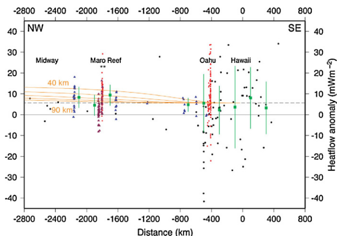
Fig. 26. Heat flow data along the Hawaiian volcano chain. The heat flow anomalies are relative to the GDH2 average oceanic model (solid gray line) and to the average heat flow for lithosphere incoming from southeast of Hawaii (dashed gray line). Predicted heatflow (orange curves) for different depths of lithosphere reheating.
