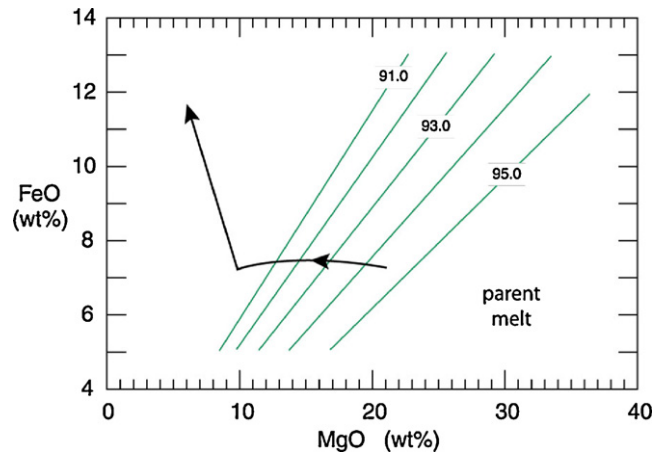
Fig. 12. Computing parental melt compositions for basalts using the olivine control line method. Green lines show the forsterite contents of olivine phenocrysts. Black line shows expected evolution in liquid composition as olivine crystallises out and \text{MgO} reduces. The quasi-horizontal black line segment is the olivine control line.
