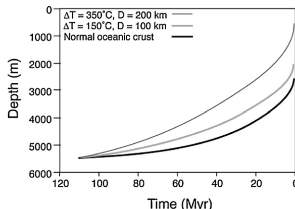
Fig. 15. Predicted subsidence curves for oceanic lithosphere that drifted away from an anomalously hot plume head.
