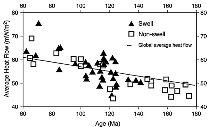
Fig. 29. Pogo heatflow data vs. crustal age for the Hawaii, Réunion, Crozet, Cape Verde and Bermuda swells (triangles) and non-swells (squares). There is no significant evidence for elevated heat flow over swells.
