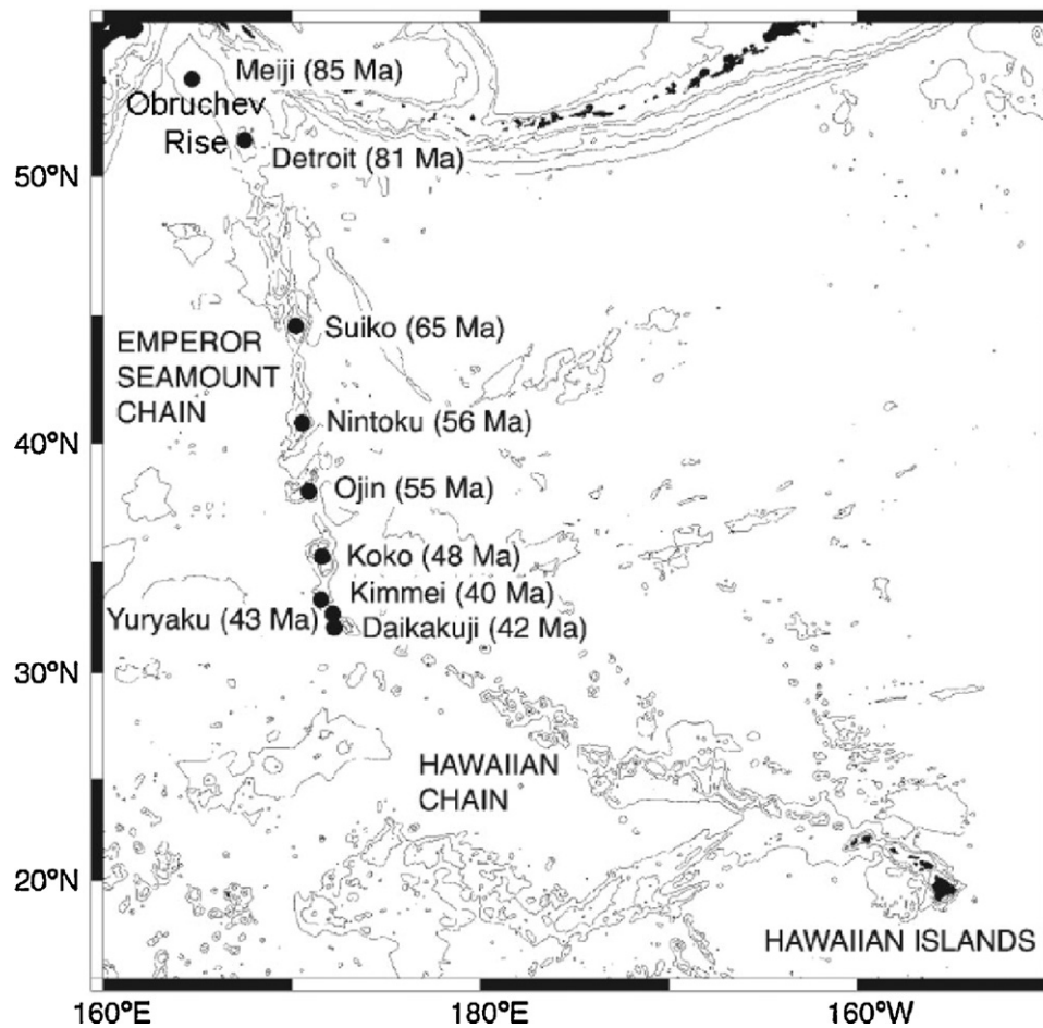
Fig. 22. Bathymetric map of the North Pacific showing the Emperor and Hawaiian volcano chains.
