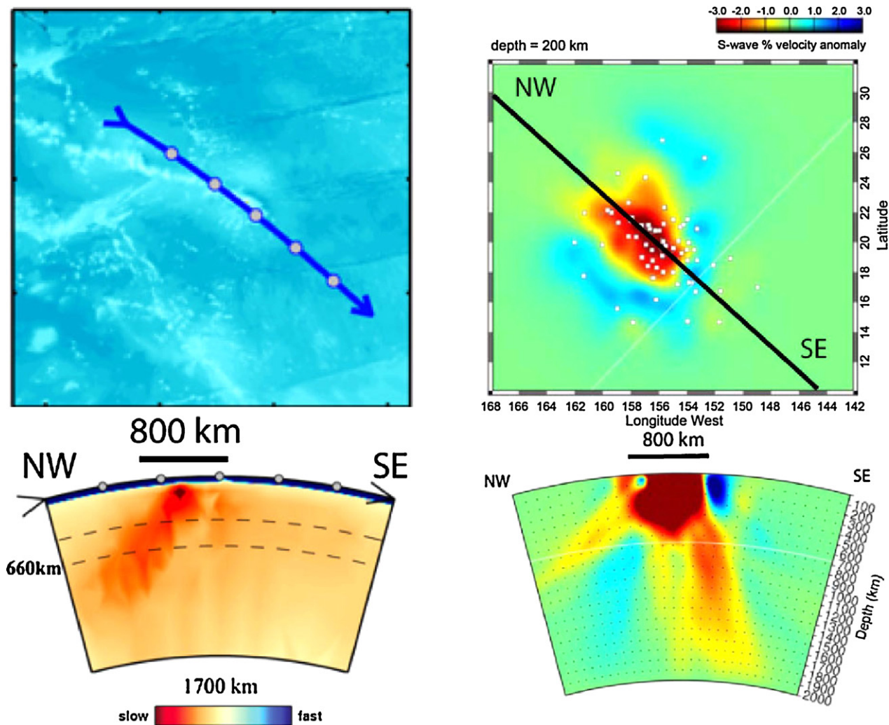
Fig. 23. Recent, relatively high-resolution tomography images of the mantle beneath the Hawaiian region. Left panels: results from the study of Li et al. (2008); right panels: results from the study of Wolfe et al. (2009).
