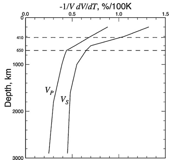
Fig. 8. Sensitivity of seismic wave speeds to temperature at different depths in Earth's mantle.
