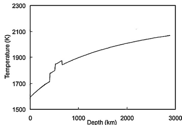
Fig. 3. Example mantle adiabat assuming a potential temperature ( T_p ) of 1590 K ( 1317^\circ\text{C} ) throughout the mantle.
