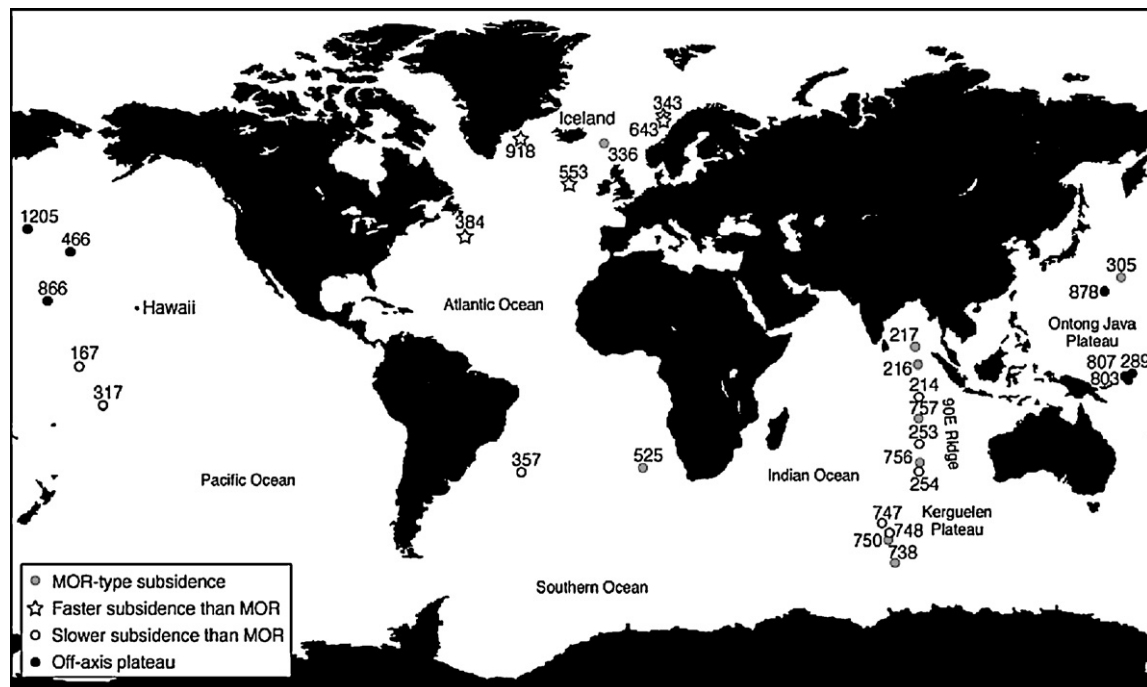
Fig. 27. Deep Sea Drilling Project and Ocean Drilling Program drill sites where the temperature of the mantle has been estimated using subsidence histories from sedimentary cores. Faster subsidence than mid-ocean ridges (MORs) indicates higher initial mantle temperatures, and slower subsidence than MORs indicates lower initial mantle temperatures.
