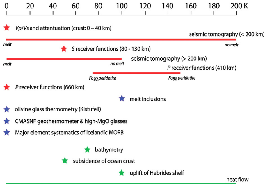
Fig. 20. Temperature-anomaly estimates for the Iceland region. Bars correspond to temperature ranges and stars to individual estimates.
