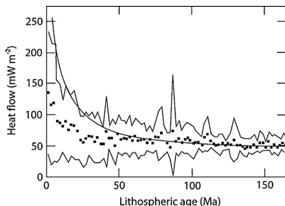
Fig. 2. Measured heat flow (dots) as a function of lithospheric age, with one-standard-deviation bounds (thick lines). Thin line shows the predicted heat flow from the GDH1 cooling model, which fits the observations best [Anderson, 2007; Stein and Stein, 1992].
