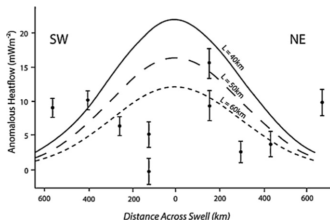
Fig. 25. Heat-flow measurements perpendicular to the Hawaiian chain compared with predictions for lithosphere thicknesses after thermal thinning of 40, 50 and 60 km [DeLaughter et al., 2005].
