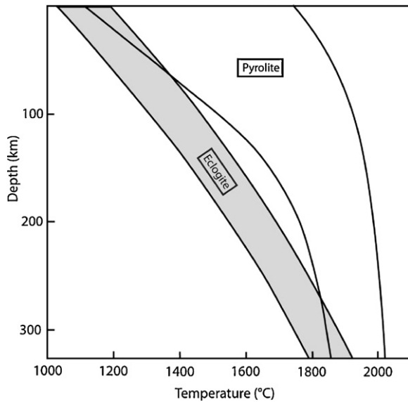
Fig. 4. Solidi and liquids of pyrolite (a proxy for peridotite) and eclogite. The eclogite solidus is up to ~500 °C lower than the pyrolite solidus in the depth range 0–250 km. The temperature difference between the liquidus and solidus of eclogite is only ~150 °C for most of the depth range for which data exist.
