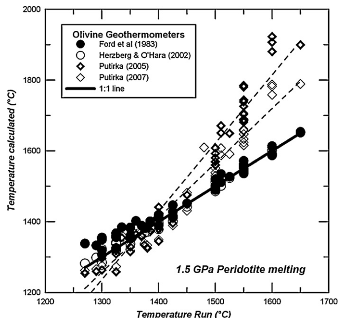
Fig. 13. Experimental vs. calculated temperatures for 55 peridotite melting and reaction experiments conducted at 1.5 GPa, and the olivine geothermometers of Ford et al. (1983), Herzberg and O'Hara (2002), Putirka (2005a) and Putirka et al. (2007).
