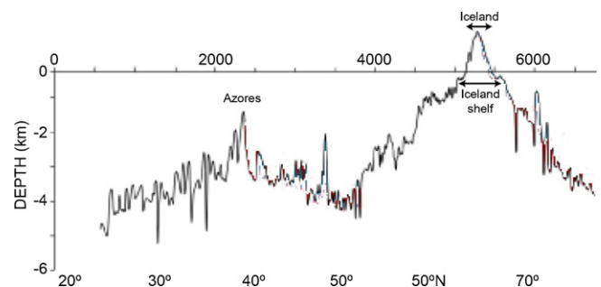
Fig. 21. Bathymetry along a profile along the Mid-Atlantic Ridge. Iceland is not an isolated topographic anomaly but simply the summit of a vast bathymetric high ~3000-km-wide that fills much of the North Atlantic.
