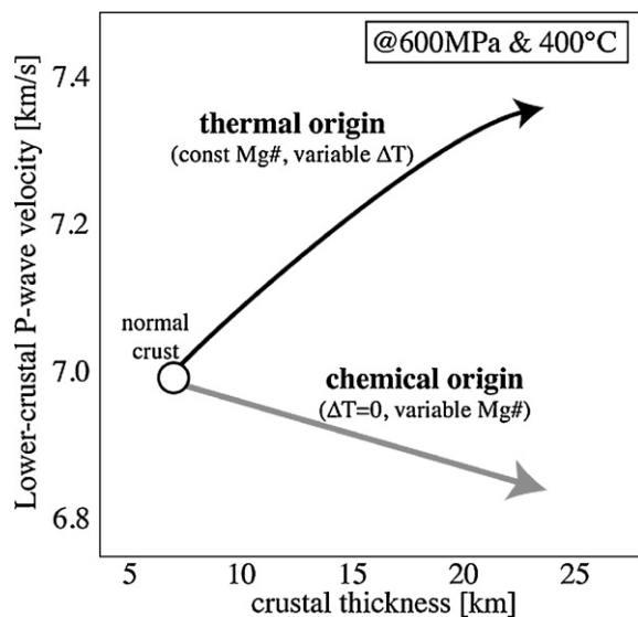
Fig. 7. Predicted relationship between crustal thickness and lower-crustal V_P at a temperature and pressure of 400 °C and 600 MPa. When thick crust is produced by anomalously hot mantle, a positive correlation results because a higher degree of melting yields magma with a higher MgO content. Thick crust can also be created by melting of fertile (low MgO) mantle, resulting in a negative correlation. Source: From Korenaga et al. (2002).
