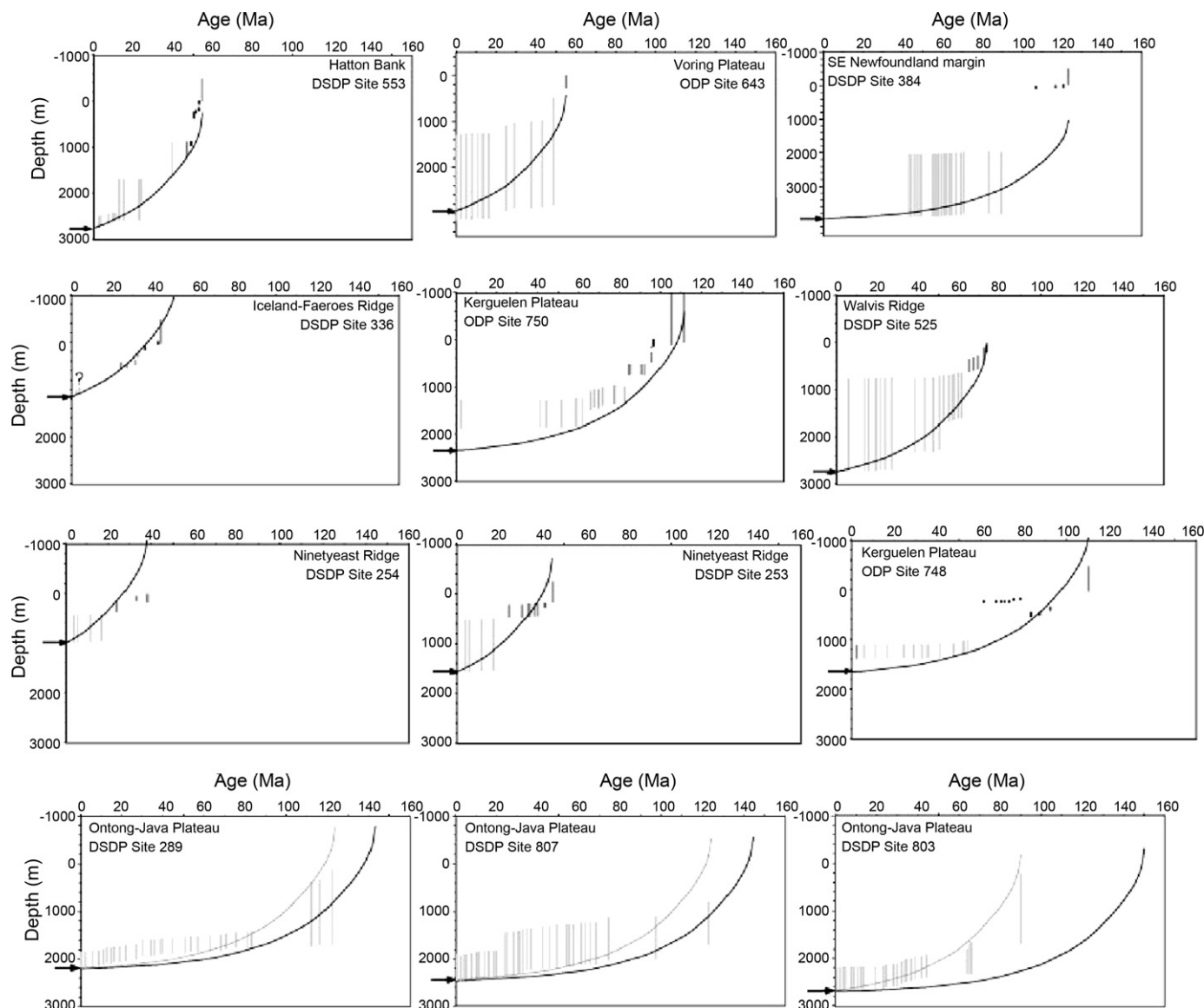
Fig. 28. Reconstructed depth-to-basement histories for a selection of sites that subsided (a) faster than average, (b) at an average rate, and (c) more slowly than average. Vertical bars show uncertainties in water depth estimates from sediments or microfossils. Black bars indicate high confidence, and gray bars low confidence. Solid curves show the predicted subsidence history for normal oceanic crust. The end points of these curves are generally known accurately. (d) Sites where volcanism occurred away from a mid-ocean ridge. The gray curves show the predicted curve for crust of the same age as the volcanic rocks (equivalent to total thermal resetting of the lithosphere), and the black curves show predicted subsidence for crust of the age of the host crust.
