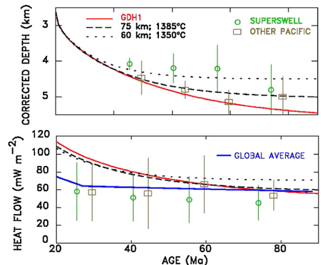
Fig. 31. Top: bathymetric depths from the Superswell and other regions of the same age in the Pacific for comparison. Bottom: heat flow observed, and predicted by thinning models [Stein and Stein, 1993].
