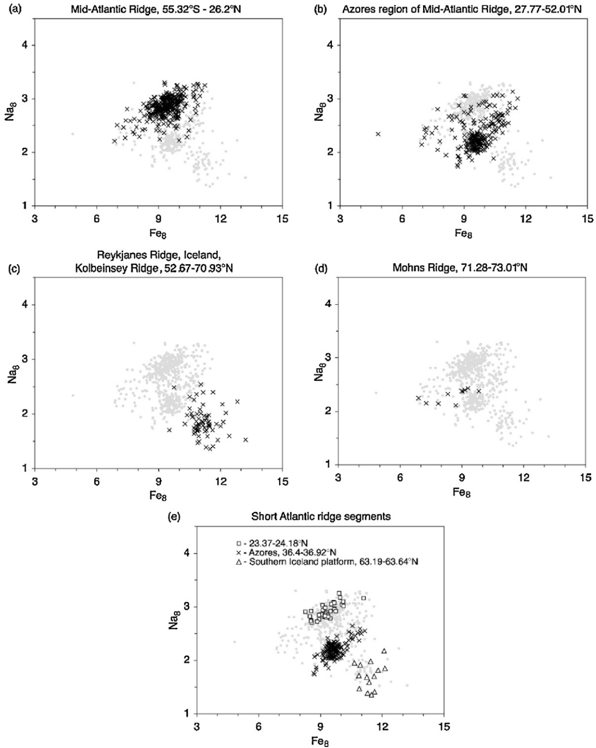
Fig. 17. Black symbols: \text{Na}_8 and \text{Fe}_8 for different segments of the Mid-Atlantic Ridge against a background of the total remaining samples (gray dots), from the southernmost end of the ridge at the Bouvet triple junction to the Mohs Ridge in the far north.
