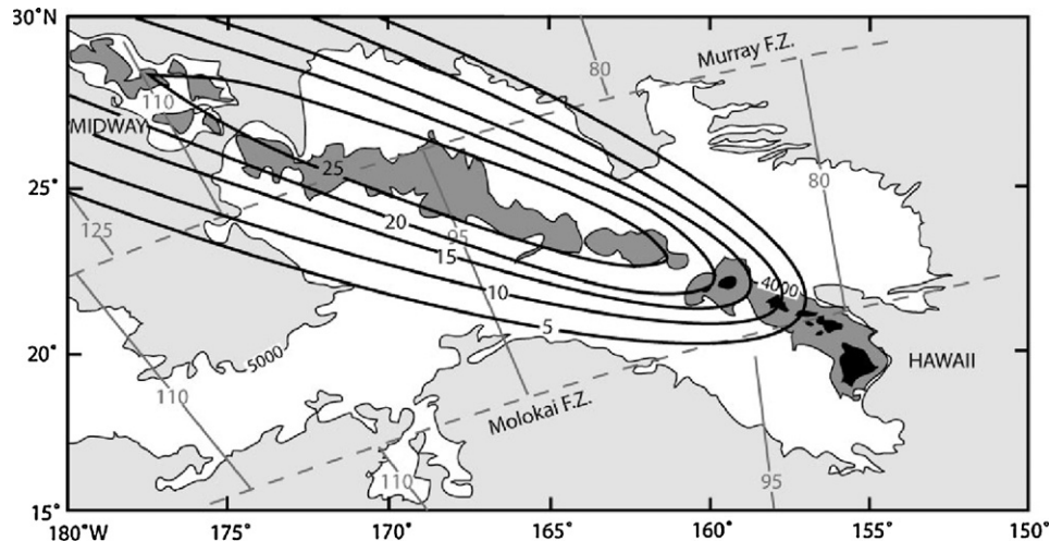
Fig. 16. Predicted heat flow anomalies for a plume that reheats the bottom of the lithosphere at Hawaii. Heat flow anomalies up to \sim 25 \text{ mW/m}^2 are predicted. Source: From Stein and Von Herzen (2007).
