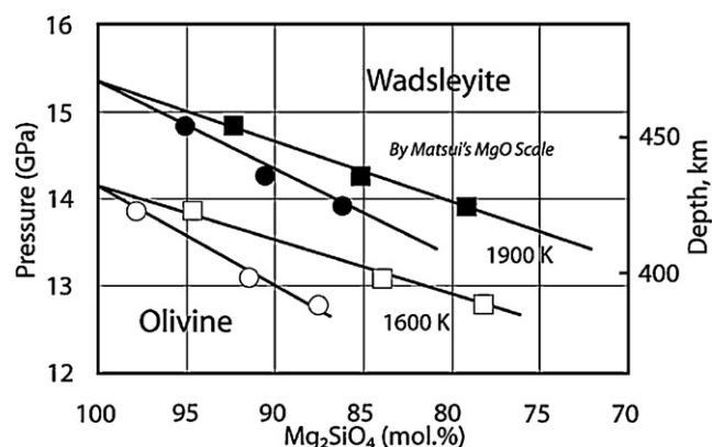
Fig. 10. Variation in the pressure of the olivine-wadsleyite phase transformation vs. composition at 1600 and 1900 °C.
