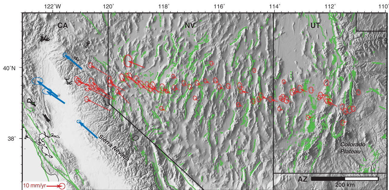
Fig. 1. GPS station velocities relative to other stations on the stable North American plate lying to the east of the network shown here. One standard deviation error ellipses are shown for each vector (27). The base map is shaded topography derived from data from the U.S. Geological Survey digital elevation model. State boundaries (CA,
