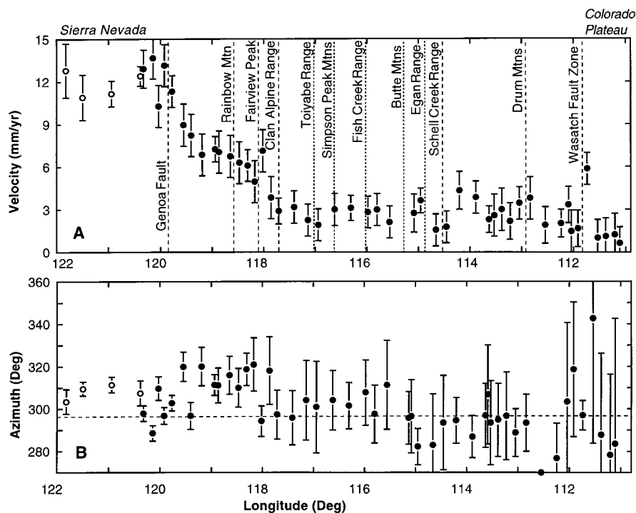
Fig. 2. Velocity magnitude (A) and azimuth measured clockwise from north (B) plotted versus longitude. Only the GPS stations along U.S. Highway 50 shown in Fig. 1 are plotted. However, the velocities of four additional continuously recording GPS stations (open circles) that lie within the stable Sierra Nevada block are shown for comparison. Error bars indicate 1 SD. Major range-bounding faults with Holocene slip (long-dashed lines) and Quaternary slip (short-dashed lines) are shown in (A), and the 308° azimuth of North America–Sierra Nevada relative motion (13) is shown by the horizontal dashed line in (B).
